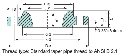
THREADED
