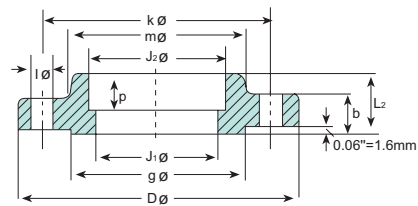
SOCKET WELDING
