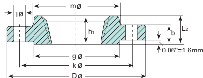
THREADED
