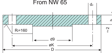
TYPE T
