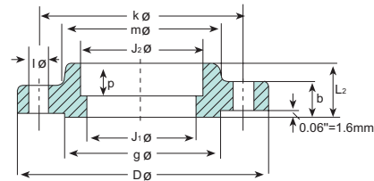
SOCKET WELDING
